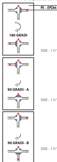
Valvola a sfera a 3 vie - PVC-U - 3 vie 3-way Series ball valves PVC-U - 3 ways
